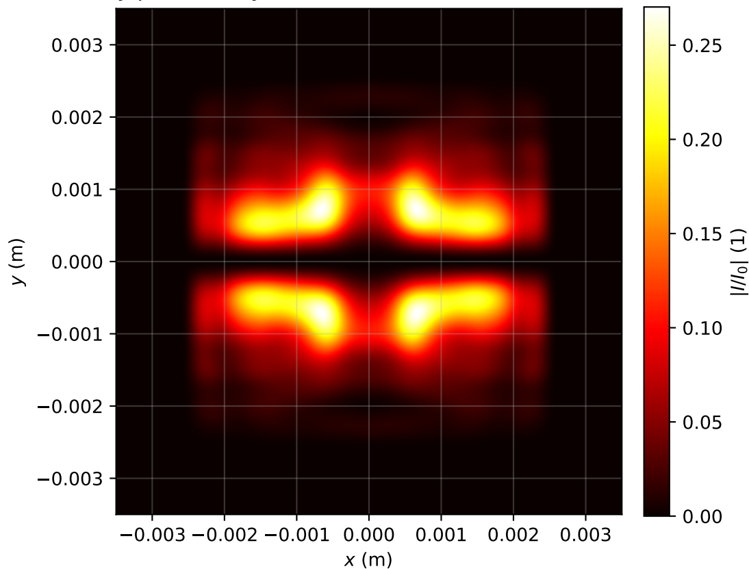
Intensity profile I(x, y, z = 3.742)/I_0 , P_{in}=4.0P_{cr} , artificial time
